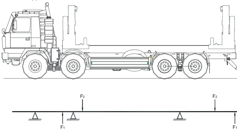
Figure 6 – Free Body Diagram for typical Truck Chassis
