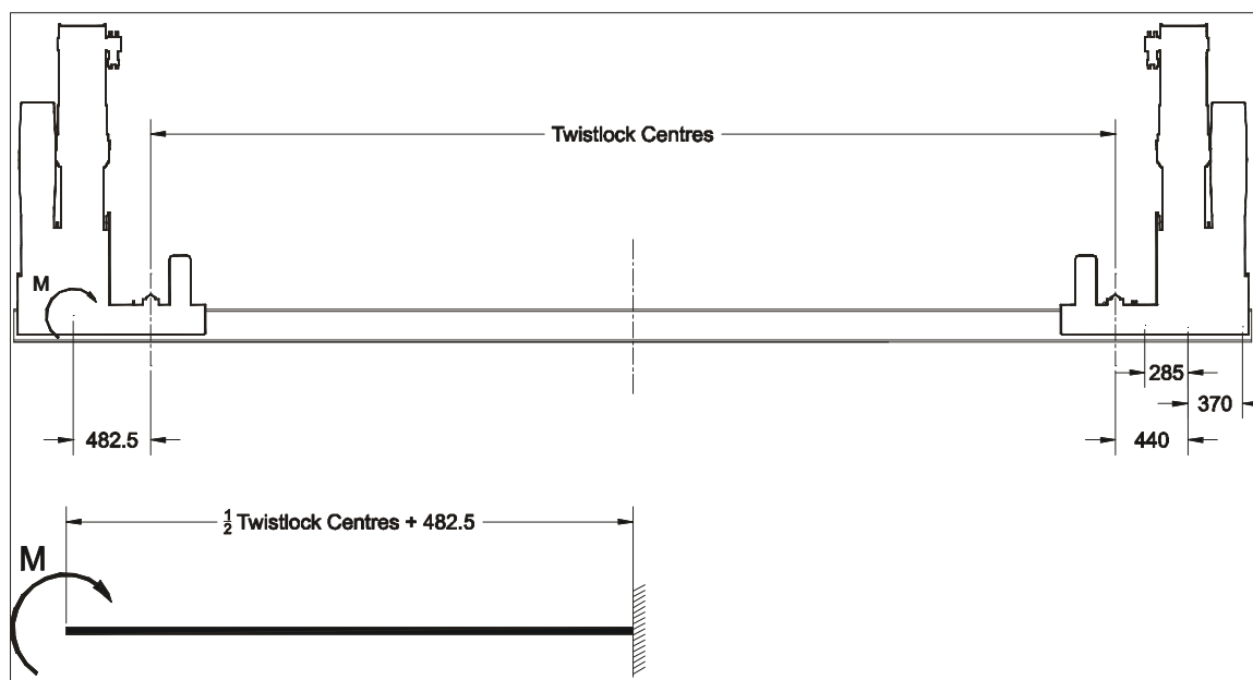
Figure 7 – Free Body Diagram for Simplified Truck Chassis
